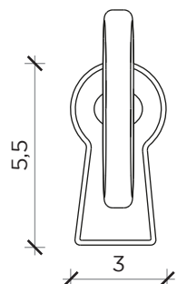
FRONTE | FRONT
