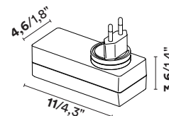
Ingombro del trasformatore M e L (plug escluso) LED driver dimensions for sizes M and L (plug excluded)
