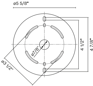
Mounting plate detail:
