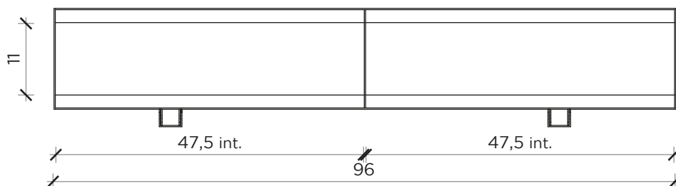
FRONTE | FRONT
