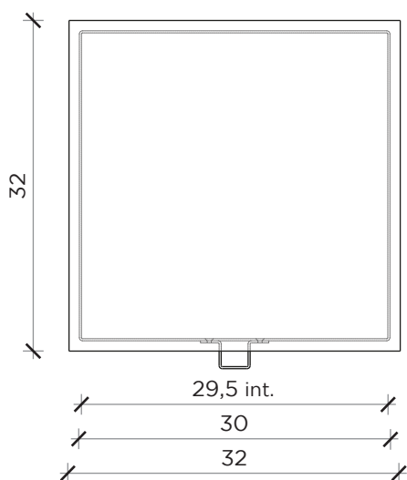
FRONTE | FRONT
