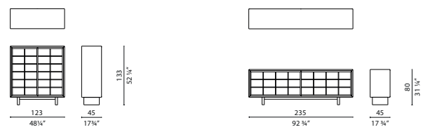
RTC1 / RTC1L
