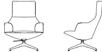
Circa Highback Swivel Chair with Armrests CIR002HBARSB W 80cm D 76cm H 105cm W 31½" D 30" H 41¼"
