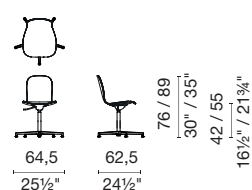
TW_5H
